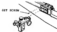
Figure 2-12. Rear sight attachment.
